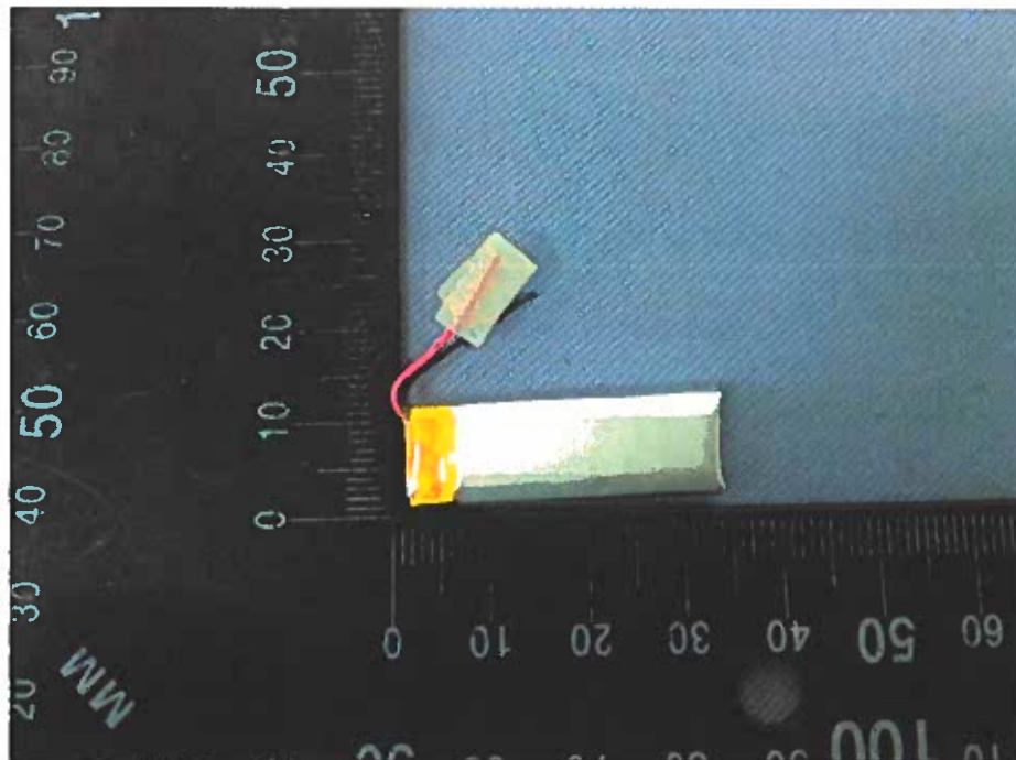
Figure 2 Overall view II of battery (电池图II)
