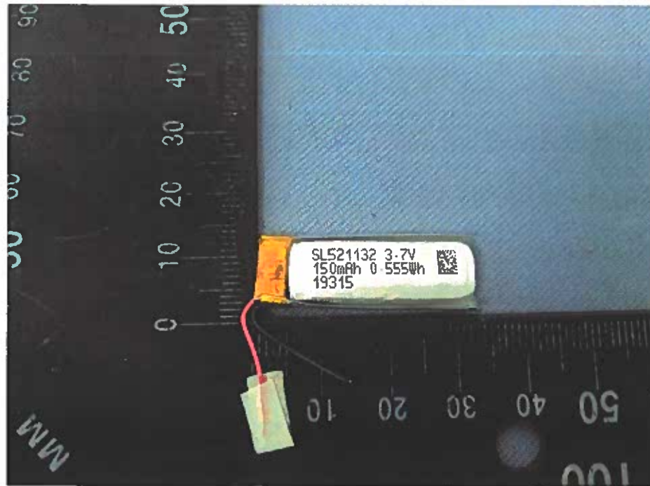
Figure 1 Overall view I of battery (电池图I)
